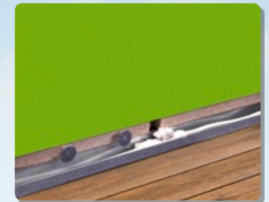
2. Measure out where the vertical cable duct is.
